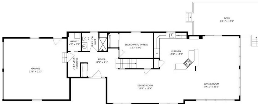
FLOOR 1
