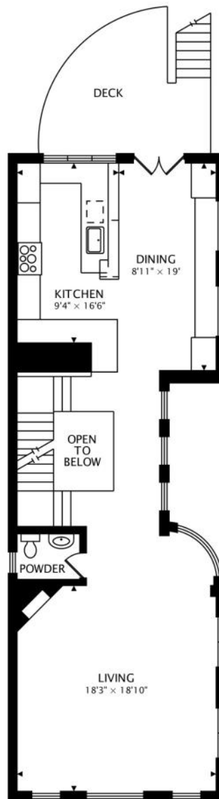
2ND LEVEL 1068 sq ft
