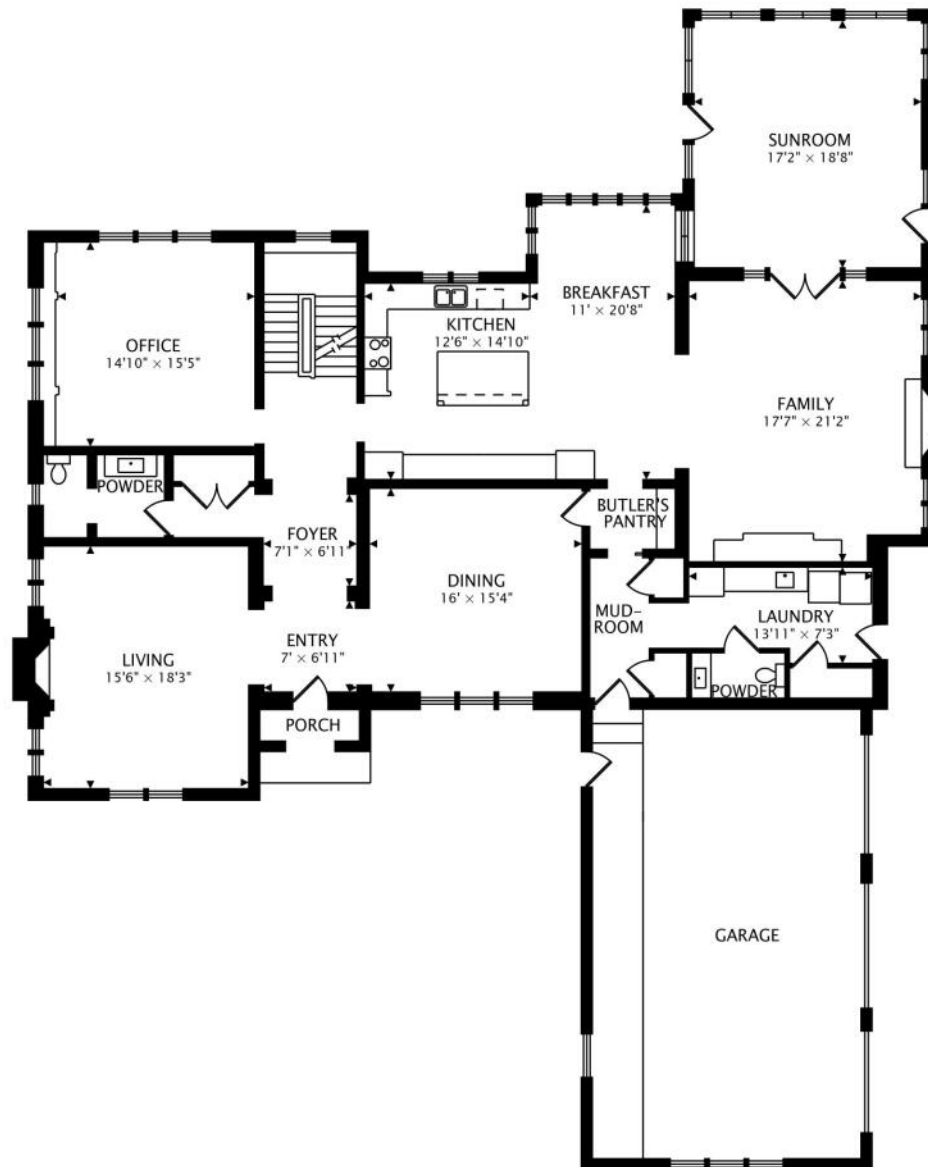
MAIN 2867 sq ft
