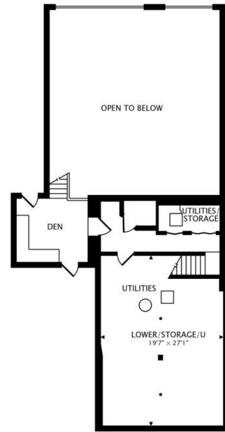
LOWER 963 sq ft BELOW GRADE
